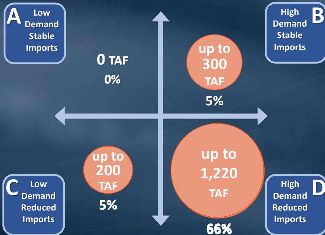
Maximum Magnitude (TAF) and Frequency (%) of a Net Shortage in Forecast Year 2045
